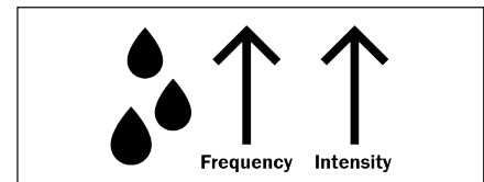
Extreme rainfall events are expected to increase in frequency and intensity under a high emissions scenario.
