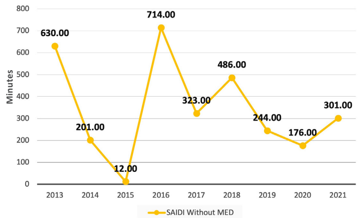
GUAM POWER AUTHORITY SAIDI WITHOUT MAJOR EVENT DAYS, 2013–2021
