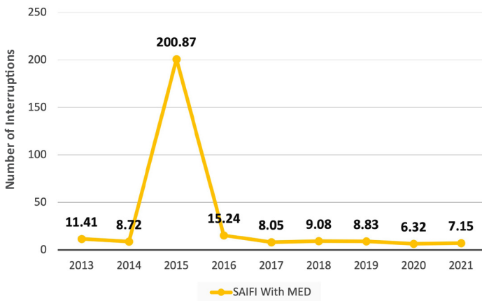
GUAM POWER AUTHORITY SAIFI WITH MAJOR EVENT DAYS, 2013–2021
