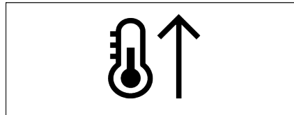
Higher daytime and nighttime temperatures by end-of-century under high emission scenarios.
