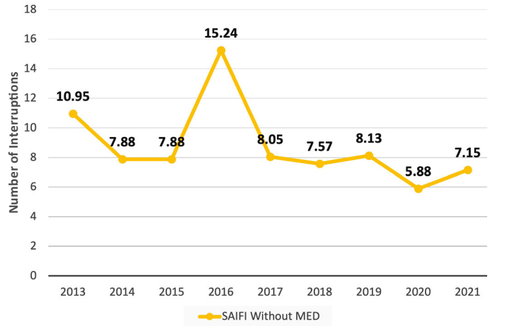
GUAM POWER AUTHORITY SAIFI WITHOUT MAJOR EVENT DAYS, 2013–2021
