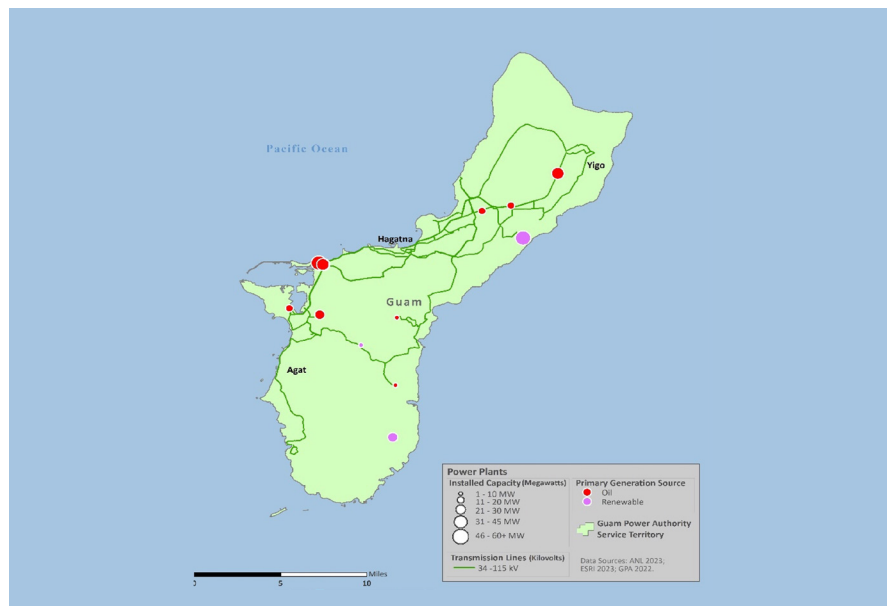
Map of electric infrastructure. Provided by Argonne National Laboratory, HIFLD Open, ESRI, and GPA.
